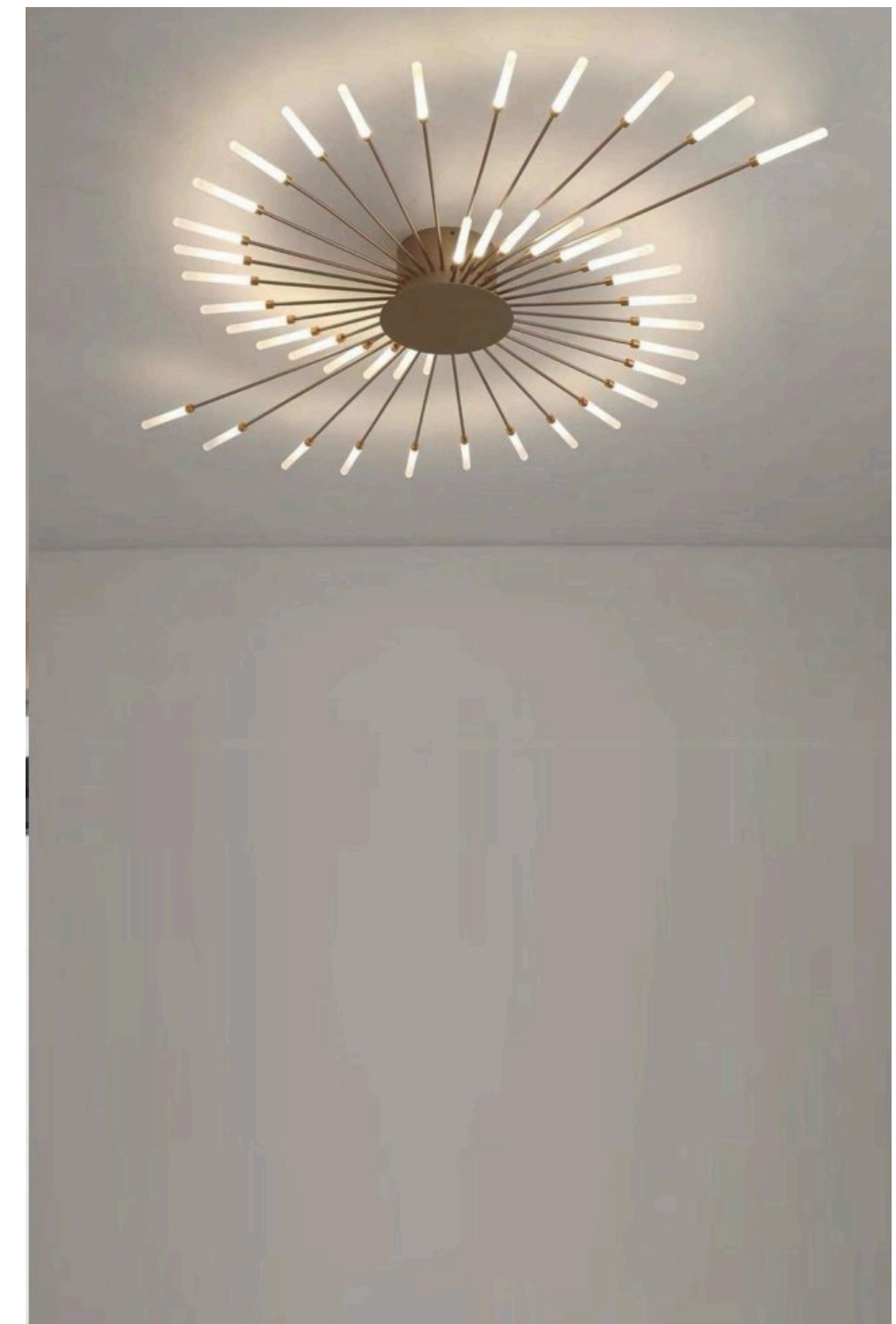
Item No : DRL 10603-21 Lamp : Led Size : H100MM X W780MM X D1280MM Finish : Gold Material : Metal
