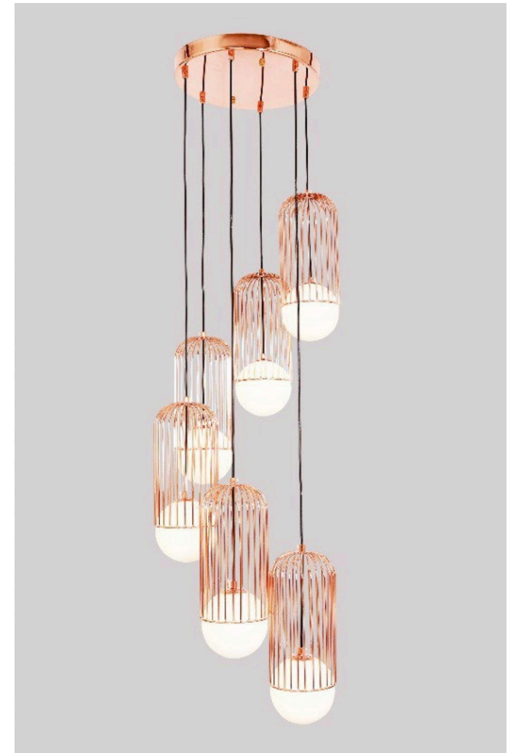
Item No : DRL 10599-6AB Lamp : 6XG9 Size : D430MM X H1800MM Finish : Antique Brass Material : Metal + Glass
