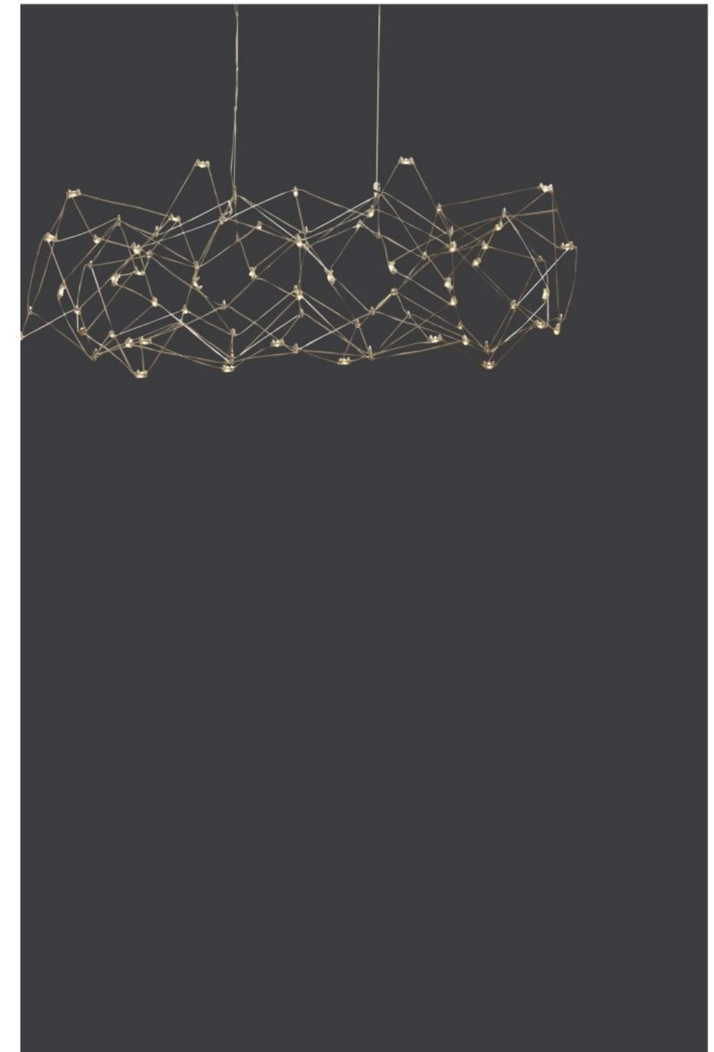
Item No : DRL 10377 Lamp : Led 48W Size : W550MMX L1300MM X H1200MM Finish : Chrome Material : Metal
