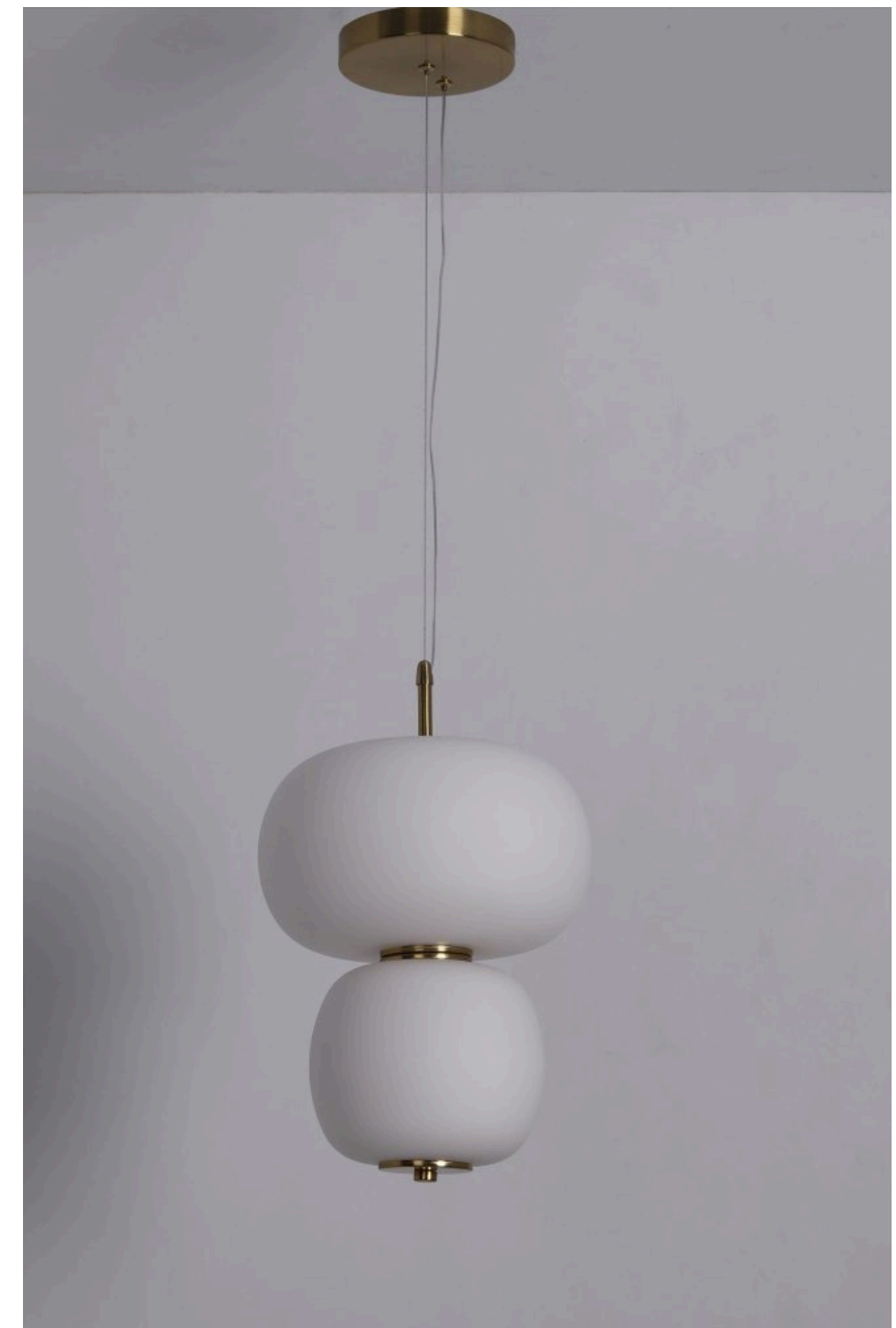
Item No : DRL 10486-1 Lamp : Led Size : D250MM X FH360MM X H1500MM Finish : Antique Brass Material : Metal + Glass
