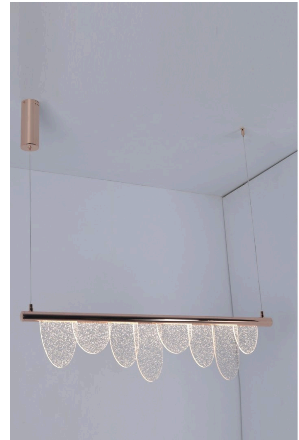
Item No : DRL 10383-900 Lamp : Led 30W Size : L900MM X W50MM X FH240MM X H2000MM Finish : French Gold Material : Metal + Acrylic
