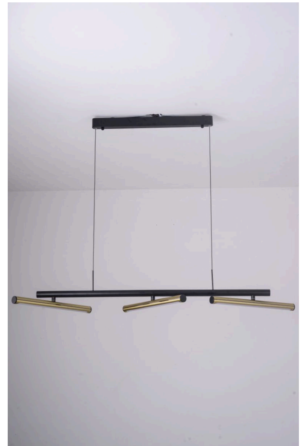
Item No : DRL 10393 Lamp : Led 48W Size : L1400MM X W40MM X H1200MM Finish : Antique Brass + Black Material : Metal + Acrylic
